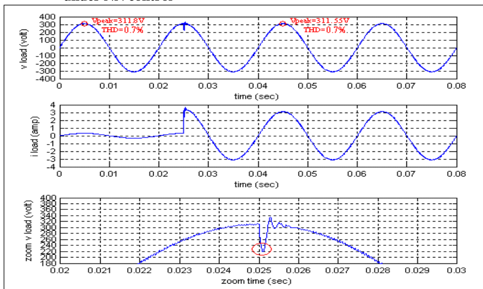
Fig.(19): Load voltage, load current at step load change (no load to full load) at t=25\text{msec} for inverter under NN control
